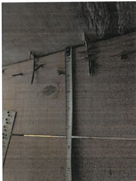
Figure 30: Roof to deck attachment.
