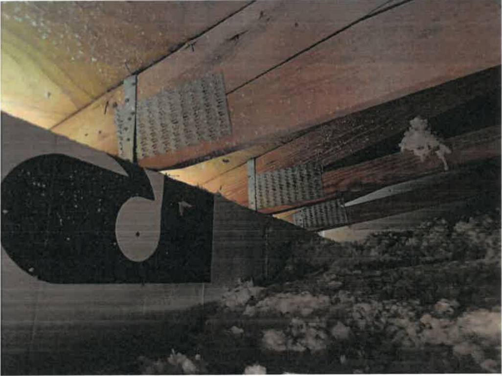
Figure 32: Roof to wall attachment.
