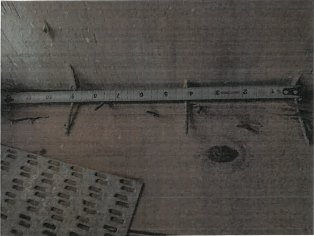
Figure 31: Roof to deck attachment.
