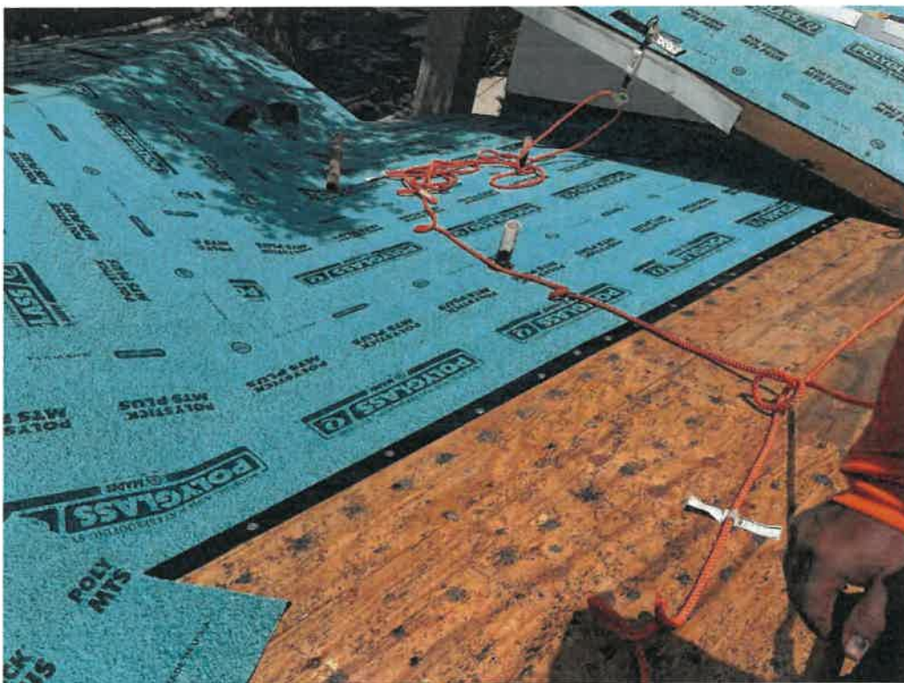
Figure 14: Roof to deck attachment.
